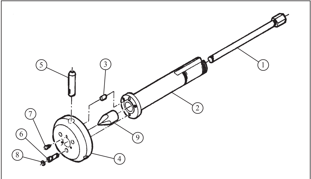
Parts List, Mandrel Assy, Elbow (P/N 06-0320)
