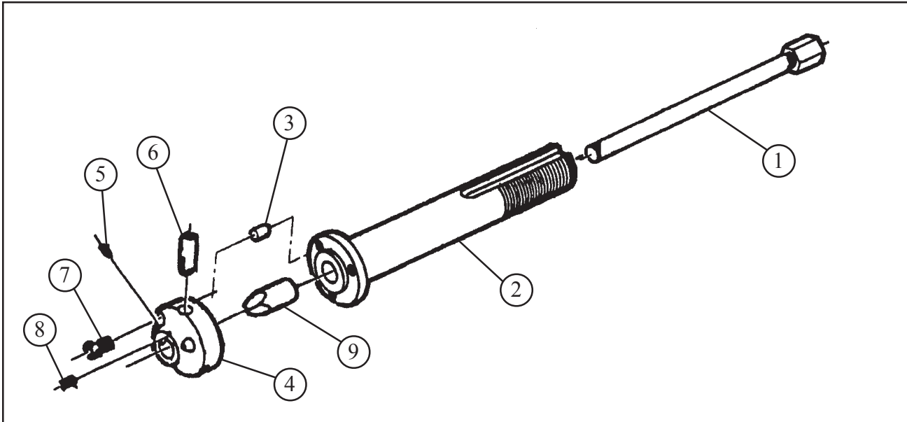
Parts List, Mandrel Assy, Elbow (P/N 06-0319)
